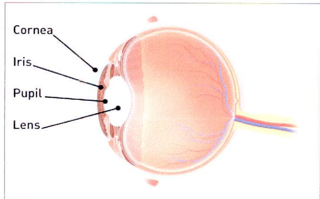
Eye anatomy
